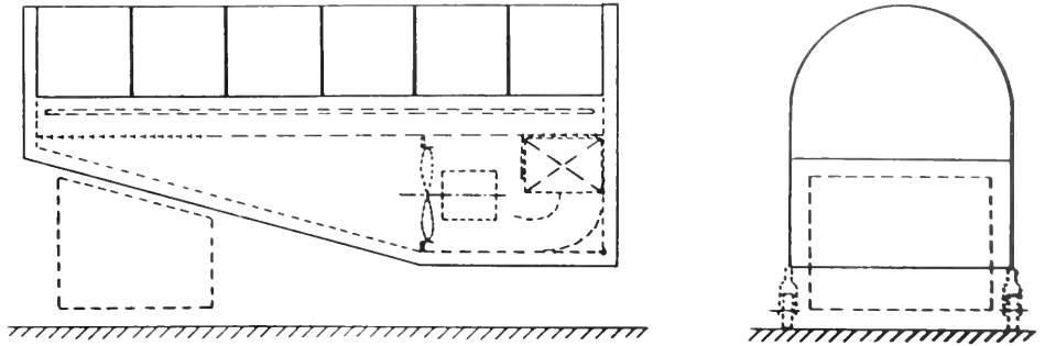
FIG. 2.—Schematic drawing of apparatus. To the right are located the fan, the cooling coils, and the heating elements. Under the left side of the apparatus is located the refrigeration system.
